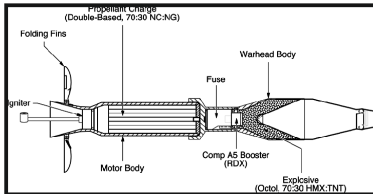
Figure 1. M 72 Anti-Tank Rocket
